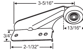
45-17
