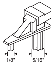
45-100 Shelf Support
