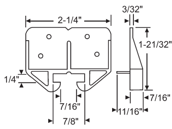
45-15 Drawer guide
