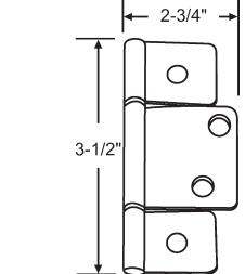
8-469 Polished Brass Extended 3 Leaf
