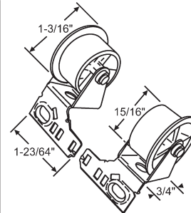
45-20A Draw Roller Set Nylon Roller
