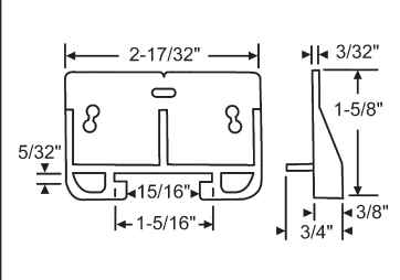
45-14 Drawer guide Old KD-14
