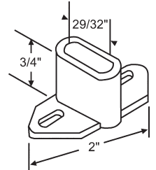
45-26 Drawer Bracket
