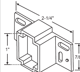
45-16 Drawer Bracket
