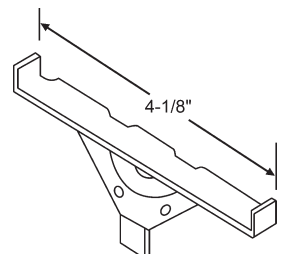
900-9382 Medicine Cabinet Shelf Bracket
