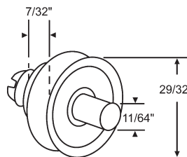
45-98 Drawer Roller with Axle
