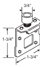
2-67 Roller Bracket
