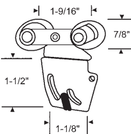
3-143 3/8" Offset
