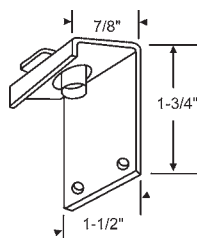
8-326 Adapter Plate
