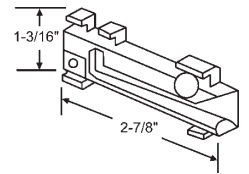
7-235A Sold as Set (1 LH, 1 RH). Nylon
