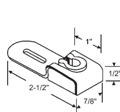
7-212 Metal with Nylon Insert
