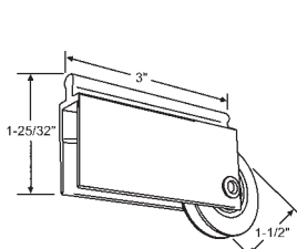
900-8319 Round-top Mirror Door Roller. Nylon Wheel
