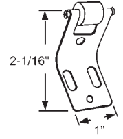
900-851 Pivot Aligner. 31/64" Dia. x 1/2" Width Nylon Roller
