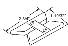
900-848 Nylon Floor Plate (Double)
