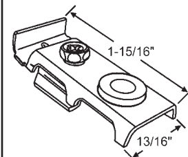
7-279 Pivot Block Clamp
