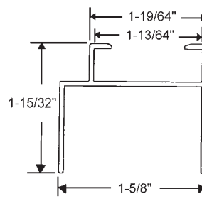
2-67 Roller Bracket
