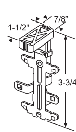
3-228 Guide Bracket
