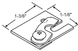
900-8986 Cam Lock Assembly
