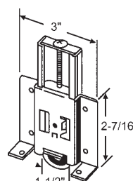
3-227 1-1/2" All Nylon Roller
