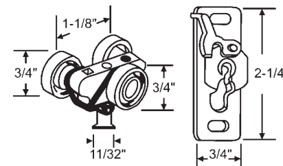
3-141 Comes with 8-226 Bracket
