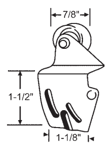
3-147 3/8" Offset
