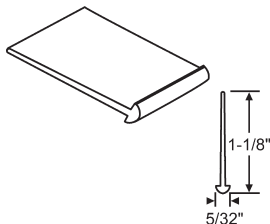
22-103 1-1/8" Shower Door Sweep
